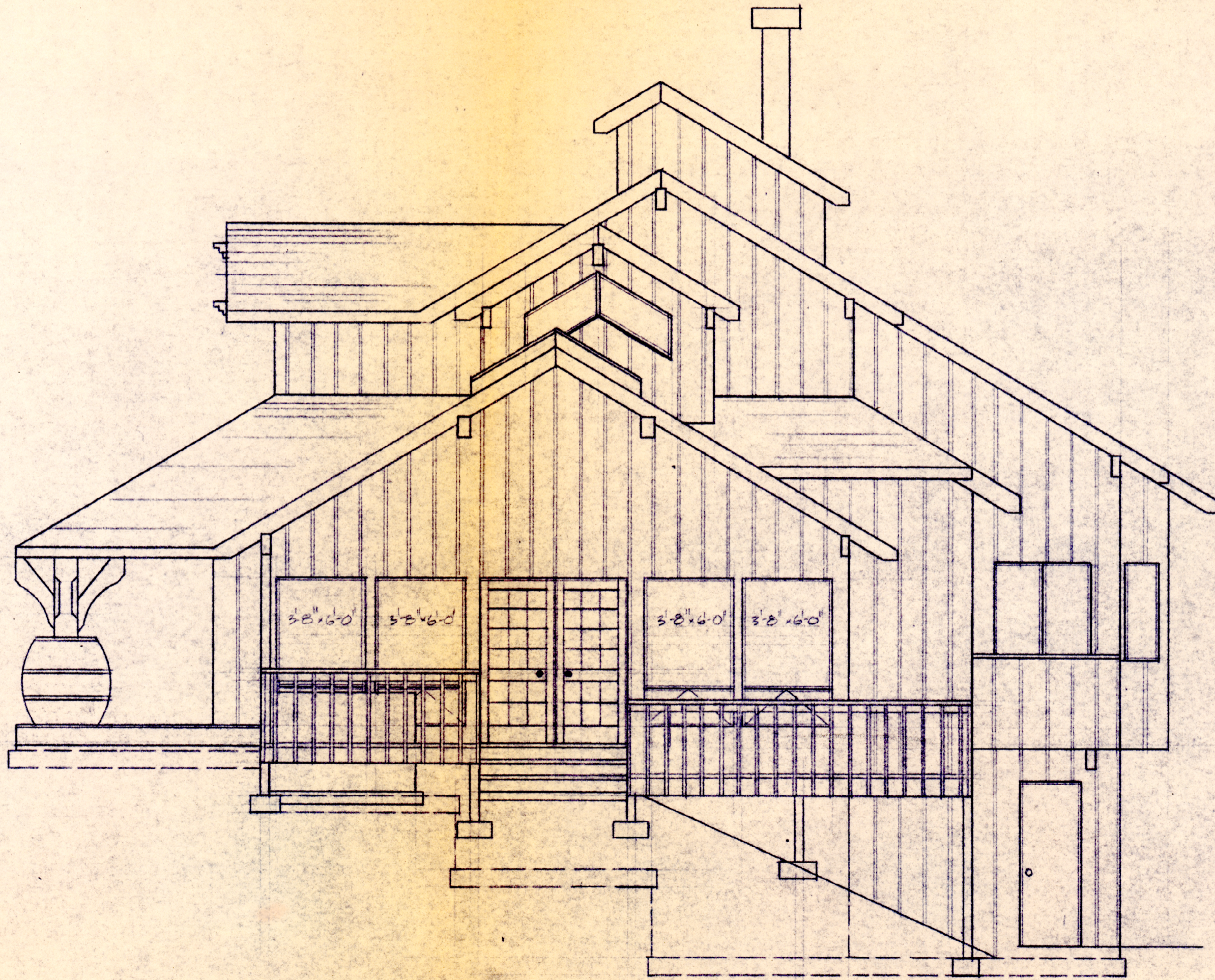
RIGHT ELEVATION (1/4" = 1'-0")
