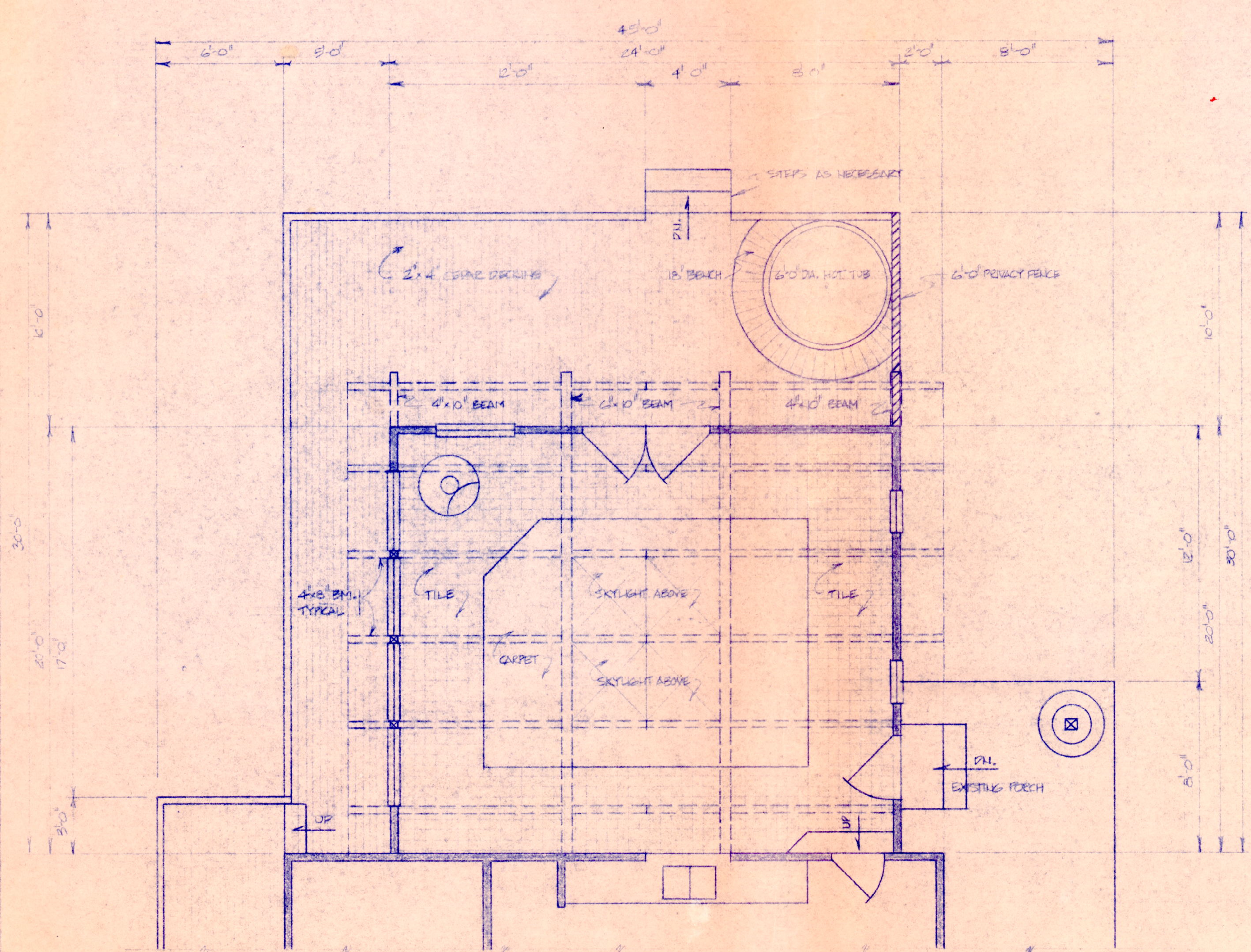
FAMILY ROOM ADDITION PLAN (1/4" = 1'-0")
