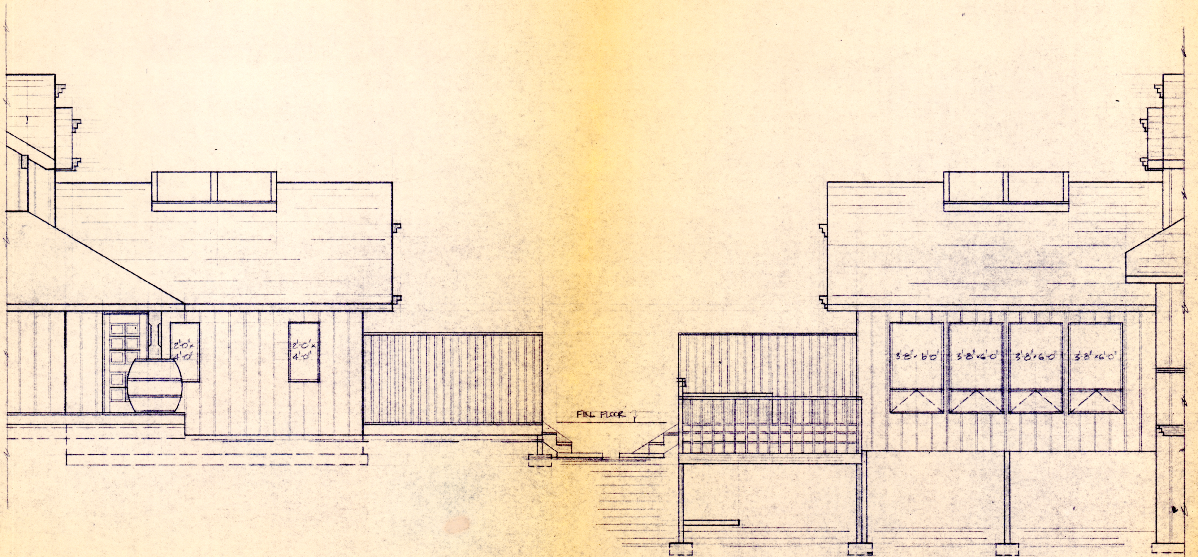
REAR ELEVATION (1/4" = 1'-0")
